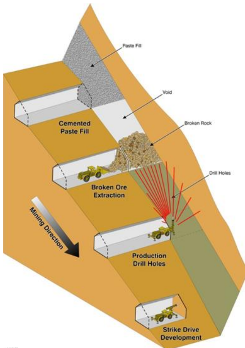
Figure 10: Dalgaranga Underground cut out of proposed stope method
