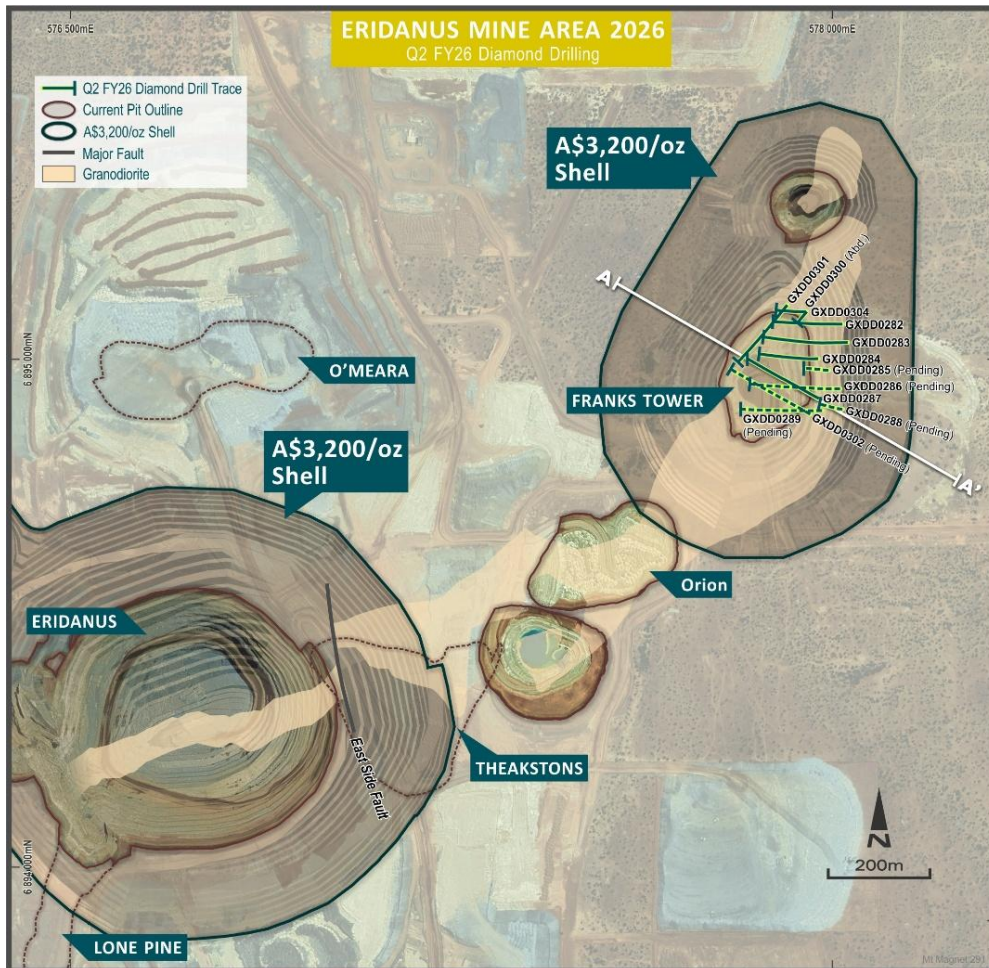
Figure 16: Franks Tower – drill hole location plan
