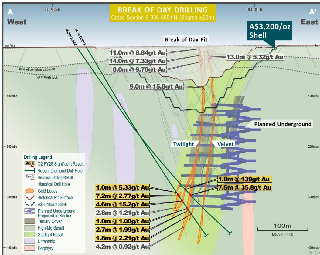
Figure 20: Break of Day – cross section showing recent results
