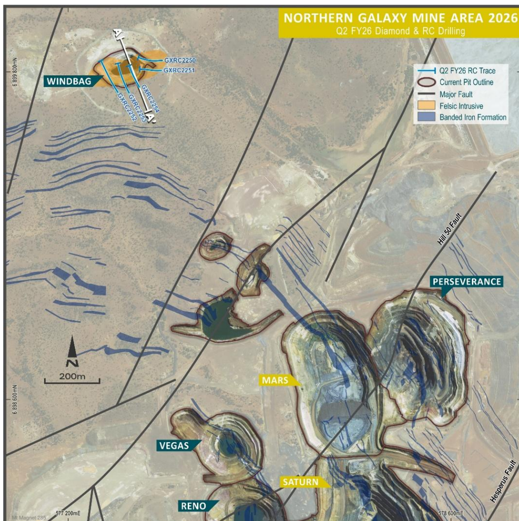
Figure 11: Windbag – drill hole location plan
