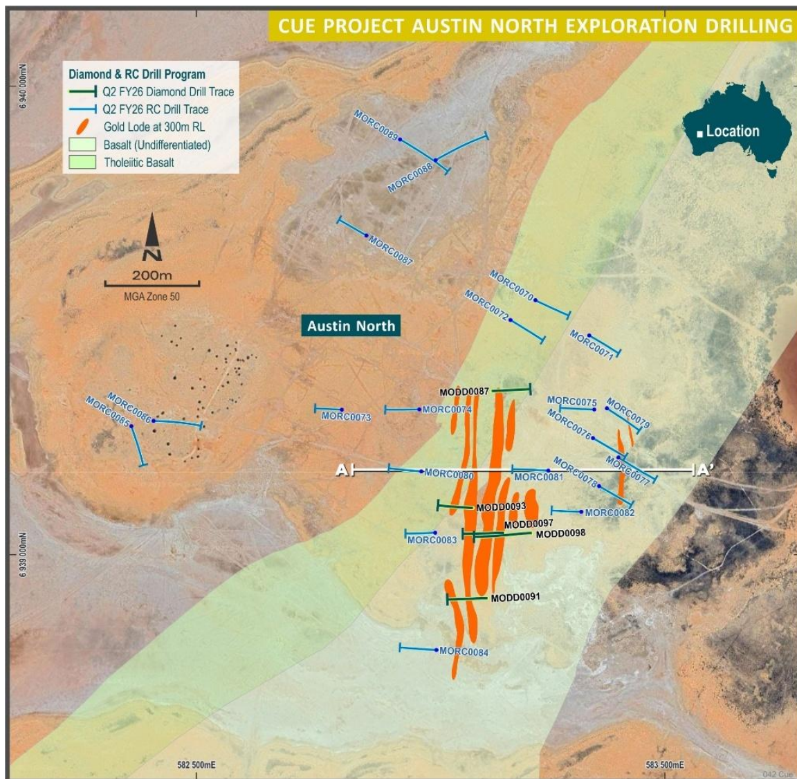
Figure 22: Austin North – drill hole location plan
