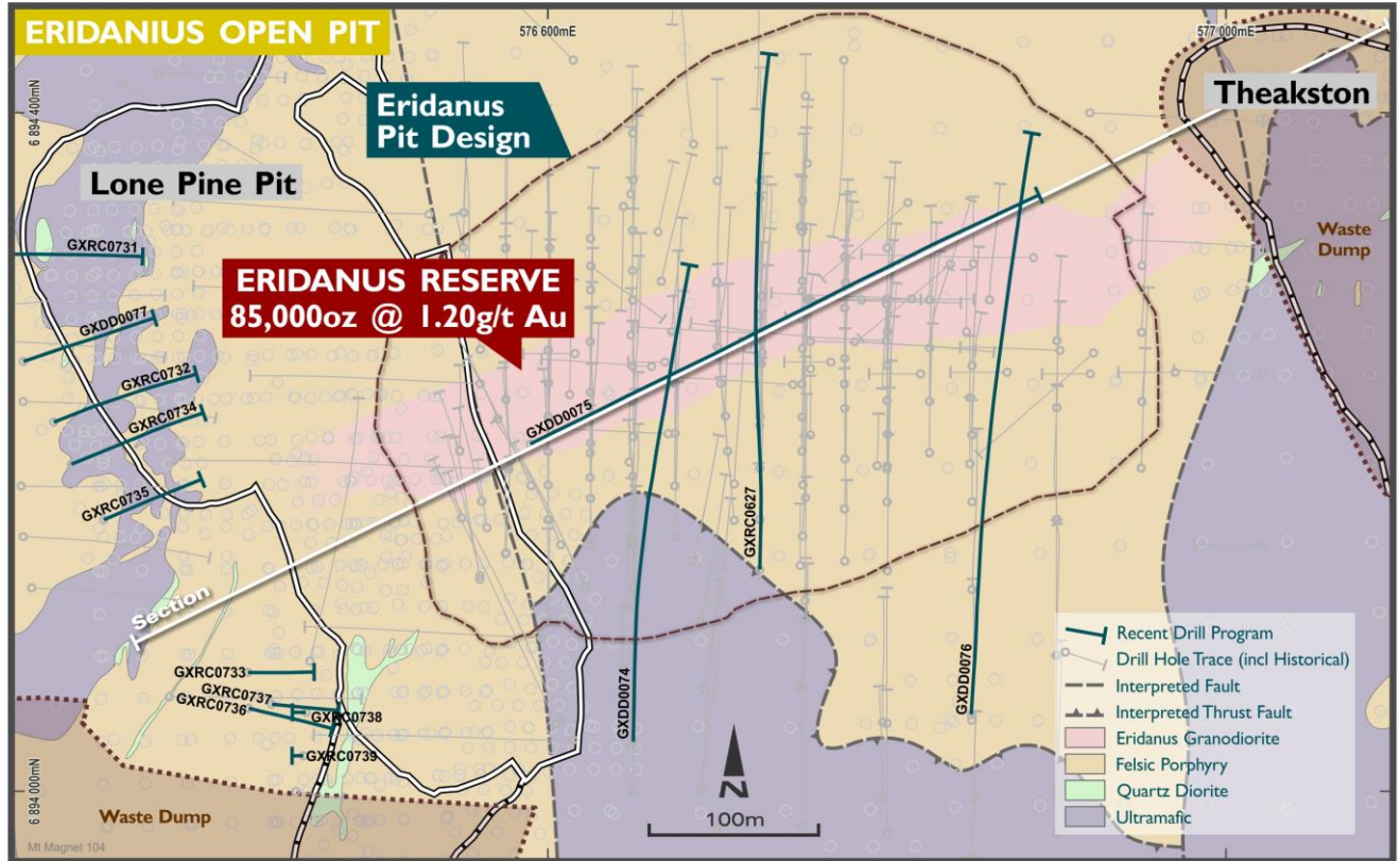
Figure 4: Lone Pine Pit and Eridanus Deeps diamond drill hole locality plan
